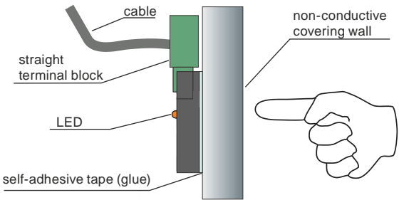
Fig. 2: CPK-C-41_1 sensor installation
