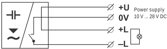
Fig. 3: Sensor wiring diagram
