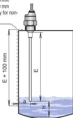
Fig. 1: Installation of level meters with rod electrode
