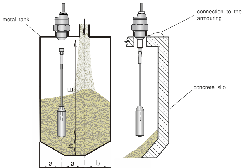
Fig. 4: Installation of level meter with rope electrode
