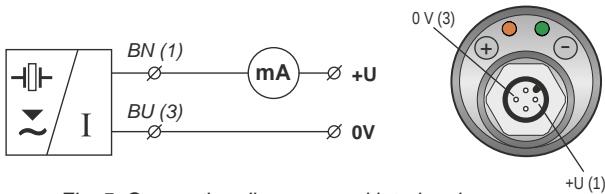
Fig. 5: Connection diagrams and interior view of connector of level meter CPC-C-35 (variant - I)
