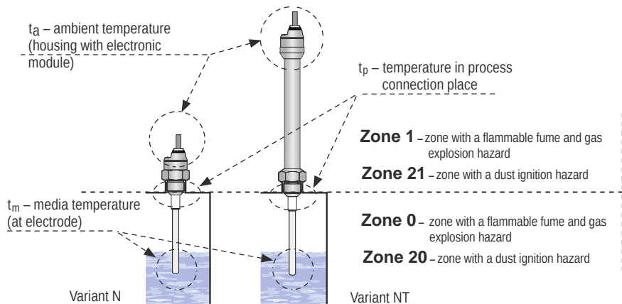
Fig. 9: Illustration of areas for temperature measurement and explosive zones
