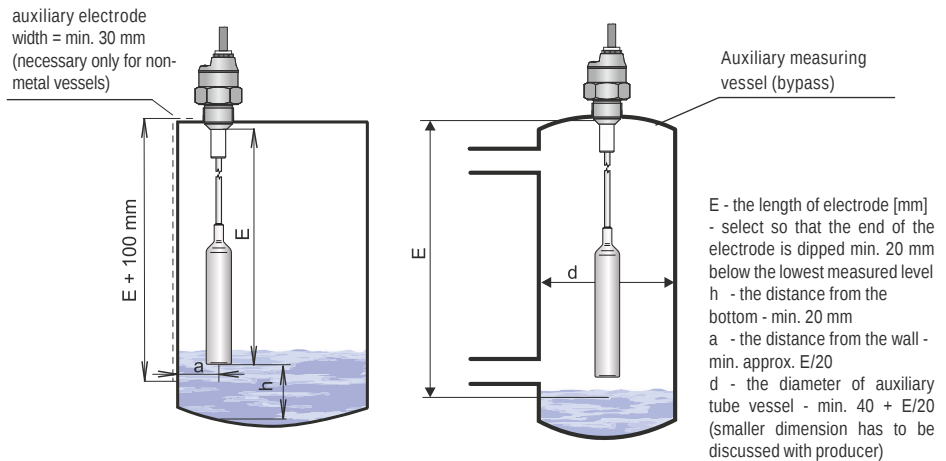
Fig. 2: Installation of level meters with rod electrode
