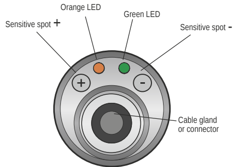
Fig. 8: Top view of level sensor
