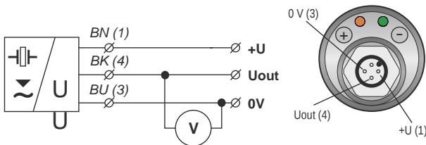
Fig. 6: Connection diagrams and interior view of connector of level meter CPC-C-35 (variant - U)
