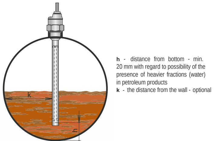
Fig. 3: Installation of level meter with reference tube
