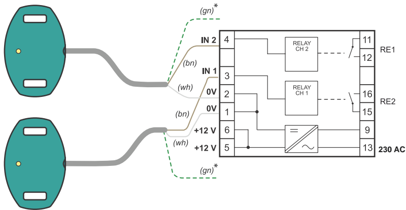
Connecting of the sensor CPK-HF-32 to the evaluation unit DSU-1222
