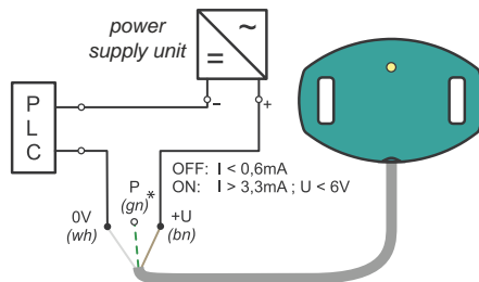
Connecting of the sensor CPK-HF-32 to the PLC logical unit
