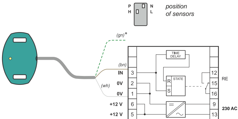
Connecting of the sensor CPK-HF-32 to the evaluation unit TDU-1211
