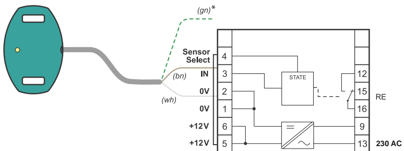
Connecting of the sensor CPK-HF-32 to the evaluation unit SSU-1211
