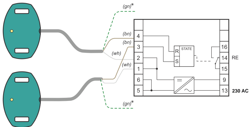
Connecting of the sensor CPK-HF-32 to the evaluation unit LCU-1221
