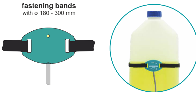
Fastening CPK-HF-32 using attachment bands
