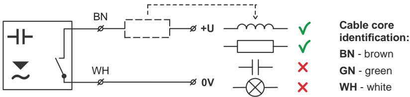
Connecting the sensor without programming wire (version M)
