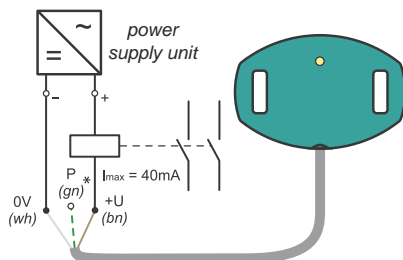
Connecting of the sensor CPK-HF-32 to the relay coil
