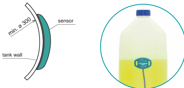
Fastening the CPK-HF-32 using self-adhesive layer
